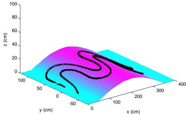
Fig. 13 Traces of front wheels for serpentine path
