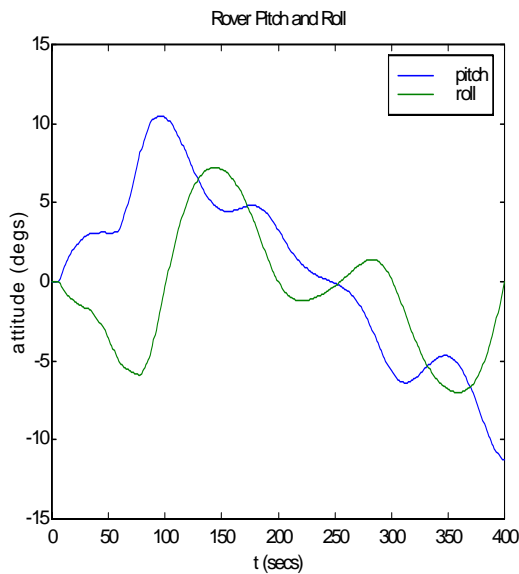
Fig. 14 Rover pitch and roll for serpentine path.
