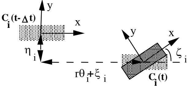
Fig. 3. Incremental motion by rolling and slip.
