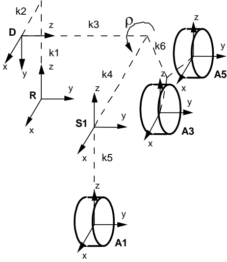
(a) Reference R, differential D, steering S1, and axle Ai (i=1,3,5) coordinate frames.
