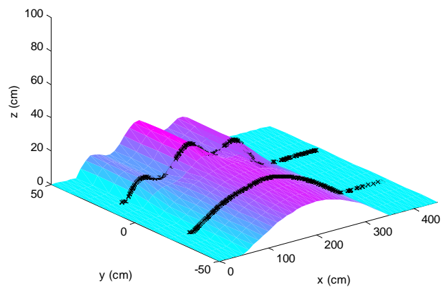
Fig. 9 Traces of front wheels over unsymmetrical wavy bump
