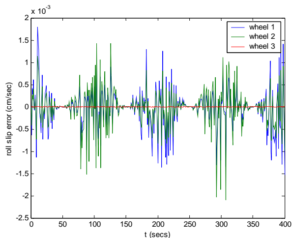
Fig. 19 Turn slip sensitivity to error in y rate
