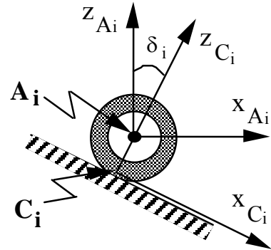
Fig. 2. Coordinate frames for terrain contact at wheel i .
