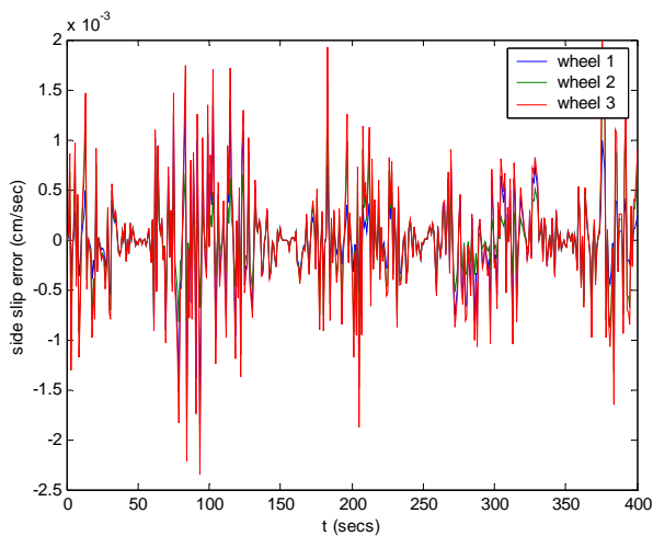
Fig. 18 Side slip sensitivity to error in y rate
