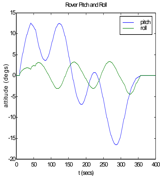
Fig. 10 Rover roll and pitch for straight path
