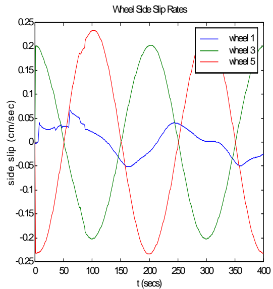
Fig. 17 Wheels side slips for left wheels
