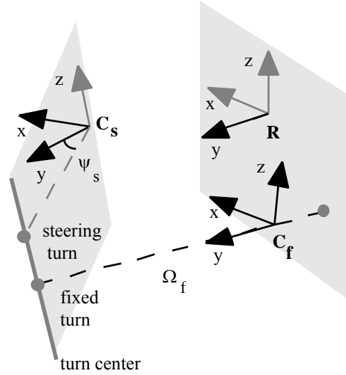
Fig. 7. Turn center corresponding to fixed wheels.
