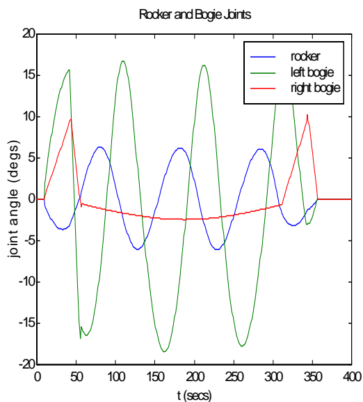
Fig. 11. Rocker and bogie joint angles for straight path.
