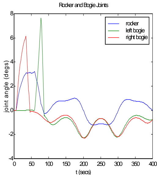
Fig. 15 Rocker and bogie joint angles for serpentine path
