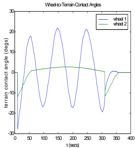
Fig. 12 Contact angle for the front wheels on straight path
