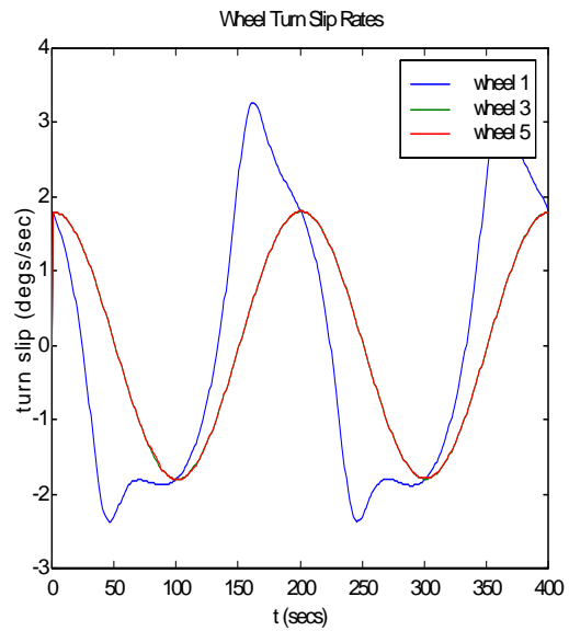
Fig. 16 Wheel turn slips for left wheels
