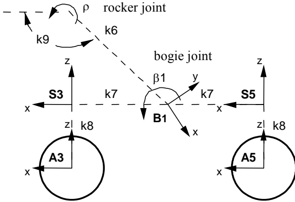
(b) Bogie B1, steering Si, and axle Ai (i=3,5) frames.
