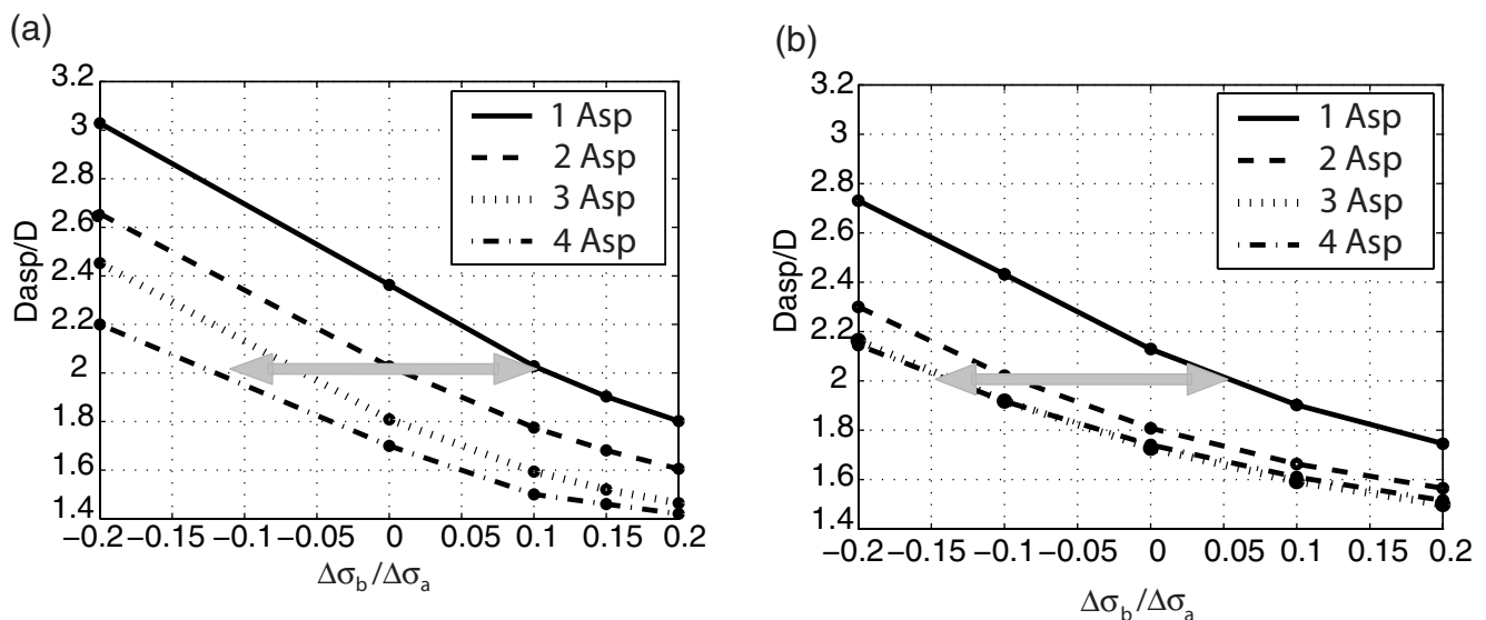
Figure 1. Average slip ratio ( D_{\text{asp}}/D ) plotted with the stress-drop ratio ( \Delta\sigma_b/\Delta\sigma_a ) for the dynamic solution of the buried earthquake (a) and surface-rupturing earthquakes (b) calculated by Dalguer et al. (2004). The arrow specifies the band of the stress-drop ratios that lies on the characterized slip model proposed by Somerville et al. (1999).
