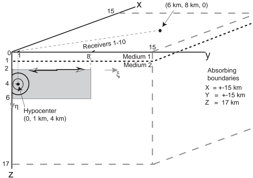
Fig. 4a Geometry for problem LOH.2
