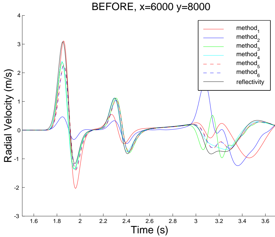
Figure 5. Initial numerical solutions for Problem UHS.1.
