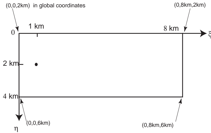
Fig 4b. Fault-surface coordinates for problem LOH.2
