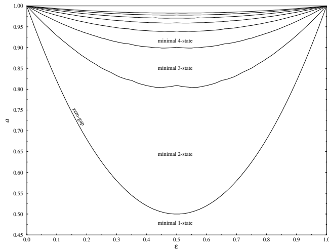
Figure 8: Convergence layers for minimal states in the piecewise linear CML. A N -minimal state is a state with N or N - 1 sites on the interface. The curve separating the layers 1-minimal state and 2-minimal state is called the zero-gap curve ( \gamma(\epsilon, a) = 0 ).
