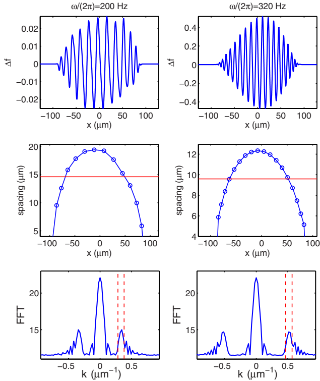
FIG. 5. (Color online) Method of averaging spacings in the inhomogeneous cloud for the NPSE model. The left and right columns of plots correspond, respectively, to \omega/(2\pi)=200 Hz and \omega/(2\pi)=320 Hz. The top row of panels shows the density deviation \Delta f from the initial density profile. The middle row of panels depicts with dots the measured spacing between maxima of \Delta f inside the cloud. The averaged spacing is shown with the red horizontal line. The bottom row of panels shows the FFT of the density |f|^2 as a function of the wave number. The vertical lines depict the estimated window of the frequencies contained in the Faraday pattern due to the nonhomogeneity in the spacings (see the middle row).
