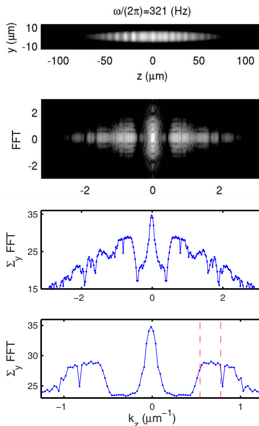
FIG. 9. (Color online) FFT analysis from the 3D numerics for \omega/(2\pi)=321 Hz. The top two panels depict, respectively, the Faraday pattern and its FFT. The third panel depicts the FFT integrated over the y direction. The bottom panel depicts the same as the third panel but the FFT is computed after adding a 2.5% noise to the density to simulate the experimental noise in the picture (notice also the difference in the depicted windows of wave numbers). The vertical lines in the last panel represent our estimated window of possible frequencies for the Faraday pattern (see the error bars in the pink squares in Fig. 2).
