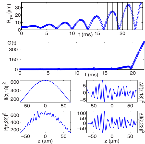
FIG. 6. (Color online) Faraday pattern from the (r, z) 3D simulations. This case corresponds to the experiment in Ref. [12], namely, a cloud of N=5 \times 10^5 ^{87}\text{Rb} atoms, trapped by \{\omega_{r,0}, \omega_z\}/(2\pi)=\{160.5, 7\} Hz with a 20% modulation of the radial confinement at a driving frequency \omega/(2\pi)=321 Hz. The top panel depicts the transverse radius of the cloud displaying impact-oscillator behavior (thin vertical lines depict the times of the snapshots shown in Fig. 7). The second panel depicts the growth of the Faraday pattern while the bottom two rows depict the r -integrated density profiles (left subpanels) and their deviation from the initial profile (right subpanels).
