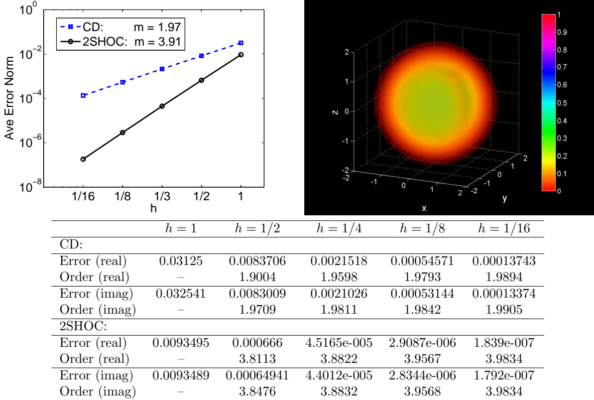
Figure 3: Top Left: Overall order of accuracy ( m ) computed from simulating the three-dimensional linear Schrödinger equation with the initial condition of Eq. (34) for the RK4+CD and RK4+2SHOC schemes. Top Right: Volumetric rendering of the modulus-squared |\Psi|^2 of the wavefunction with h = 1/16 at t = 0 (displayed on a smaller grid than used in the simulations). Bottom: Table of error values and order of accuracy values for each spatial step h . The parameters used for the solution are s = 0 , and a = 1 . The solution is integrated to an end time of t = 10 with a time-step size of k = 0.0005 .
