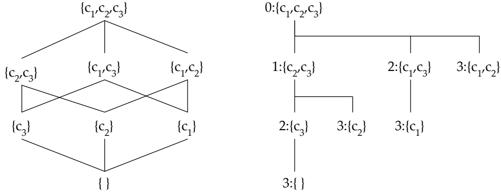
Figure 1 Boolean lattice and binomial spanning tree for |C| = 3 .
