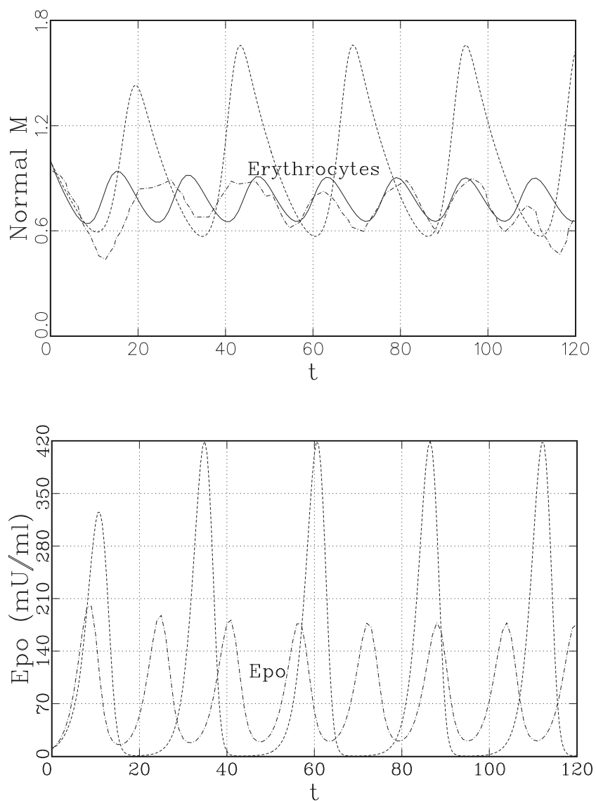
FIG. 2. Top : data from Orr et al. (1968) on the circulating erythrocytes of a rabbit suffering from autoimmune haemolytic anemia (dashed–dotted line) superimposed on the simulation of equations (2.1)–(2.8) with variable velocity V(H) and parameter values established at the beginning of Section 4 (full line) and the corresponding model with constant velocity, V(H) = 1 (dashed line). Notice the increase in amplitude when the velocity is constant, and the much better fit to the data obtained by allowing the velocity to vary. Bottom : hormone levels corresponding to the simulations of the top figure. Variable velocity (dashed–dotted line) and constant velocity (dashed line). Notice the effect of the variable velocity on both amplitude and period of the oscillations, as discussed in Section 4.
