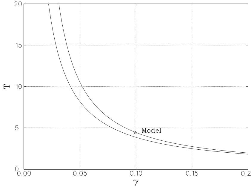
FIG. 1. Stability diagram for equation (3.25) in the case of constant maturation velocity (lower curve, \alpha_1 = 0 ) and positive velocity (upper curve, \alpha_1 > 0 ). The bullet labelled ‘Model’ corresponds to the parameter values derived in Section 4 for the anaemic rabbit, with simulations displayed in Fig. 2.
