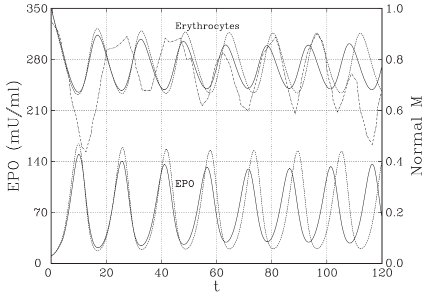
FIG. 3. The model (2.10) with moving boundary conditions, \mu_F = 4.1 and \gamma = 0.065 , (dashed line), is fitted to and compared with the data of Orr et al. (1968) which is given by the dashed-dotted line. The model (2.11) with \nu_F = 50 and other parameters matching those for (2.10) is shown with a solid line.
