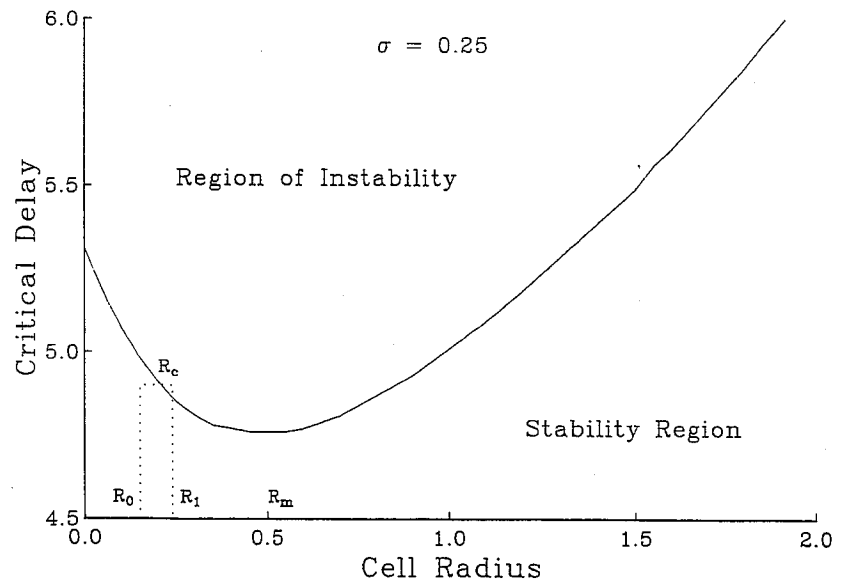
FIG. 5. Graph of the critical delay versus the cell radius R .
